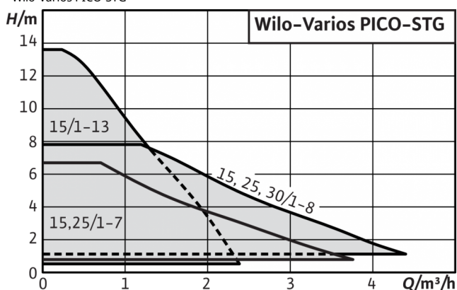
Wilo-Varios PICO-STG
